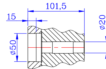
Spindle Hole
