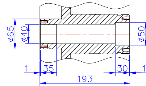
SPINDLE HOLE
